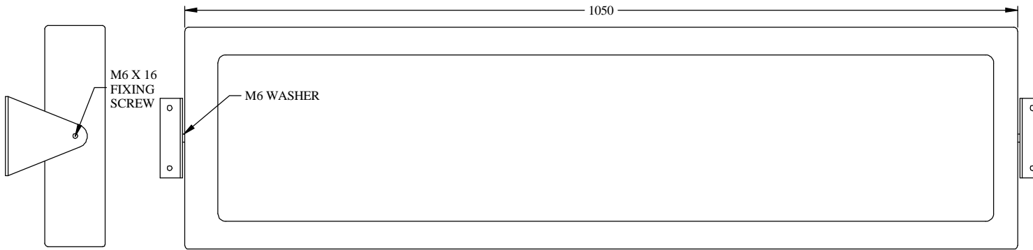
FRONT VIEW
